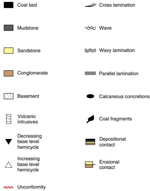
Supplementary Figure 1. Stratigraphic sections of Santa Fe de Antioquia and San Jerónimo Sub-basin
