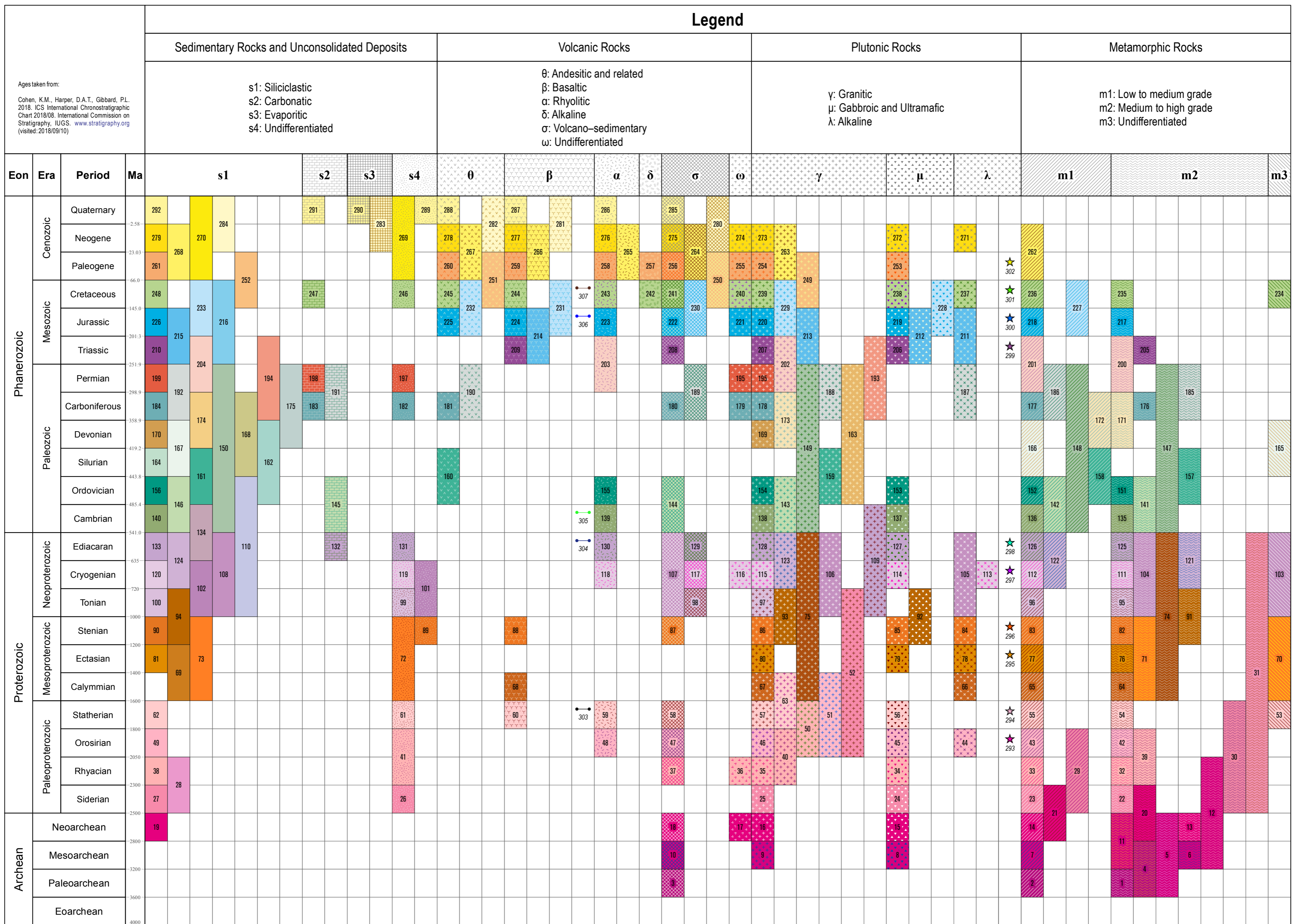
Legend of the Geological Map of South America at a Scale of 1:5M
